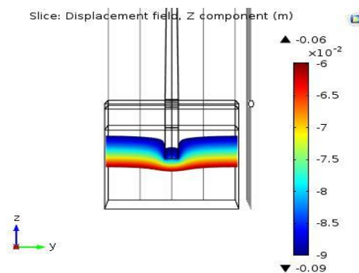
Figure 10 Vertical displacements at Z direction under the pile
