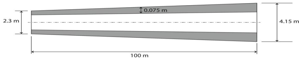
Figure 3 Sectional dimensions of the tower
